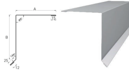
Ortgang
